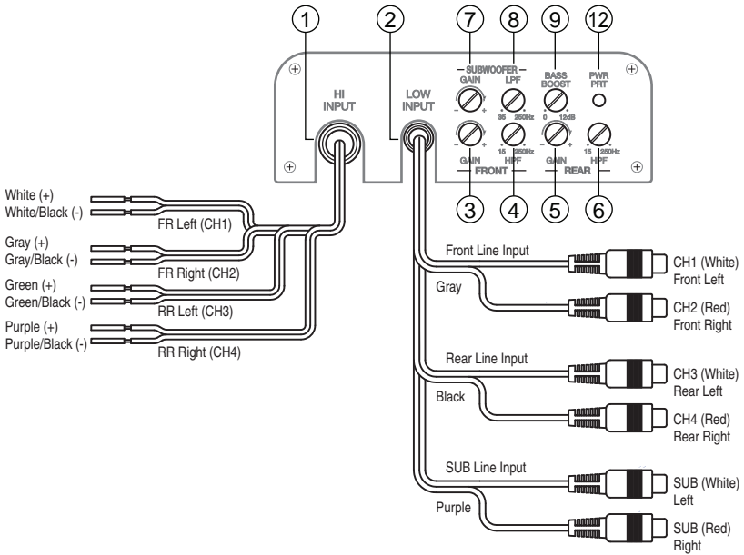
XC2510 controls and input connections
